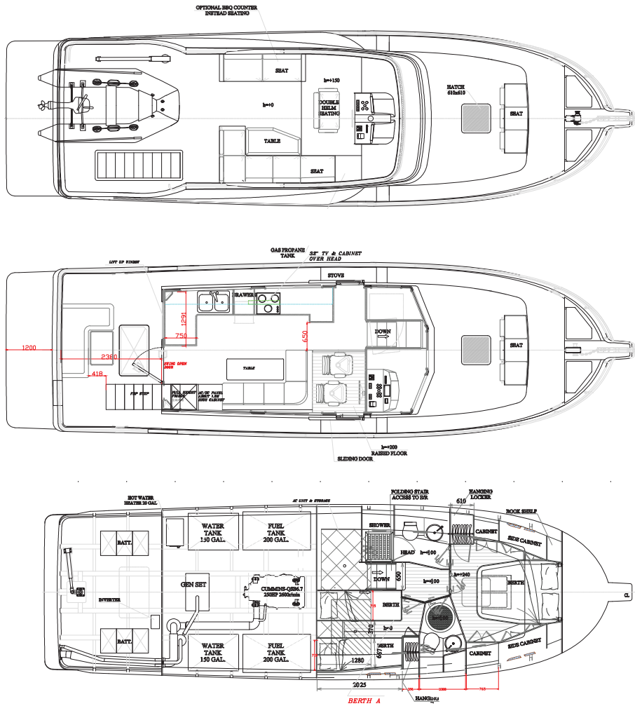
Two cabin and two bathroom layout
